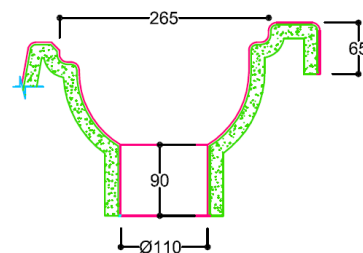
SECTION C DRAIN
